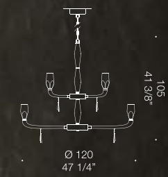
FLUTE K12+6 18xMAX 33W G9
