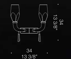
FLUTE A2 2xMAX 33W G9
