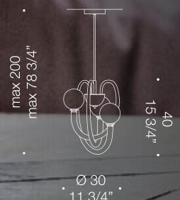
KNOT S 3x MAX 60W G9
