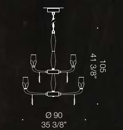
FLUTE K8+6 14xMAX 33W G9
