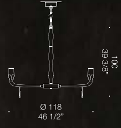
FLUTE K12 12xMAX 33W G9
